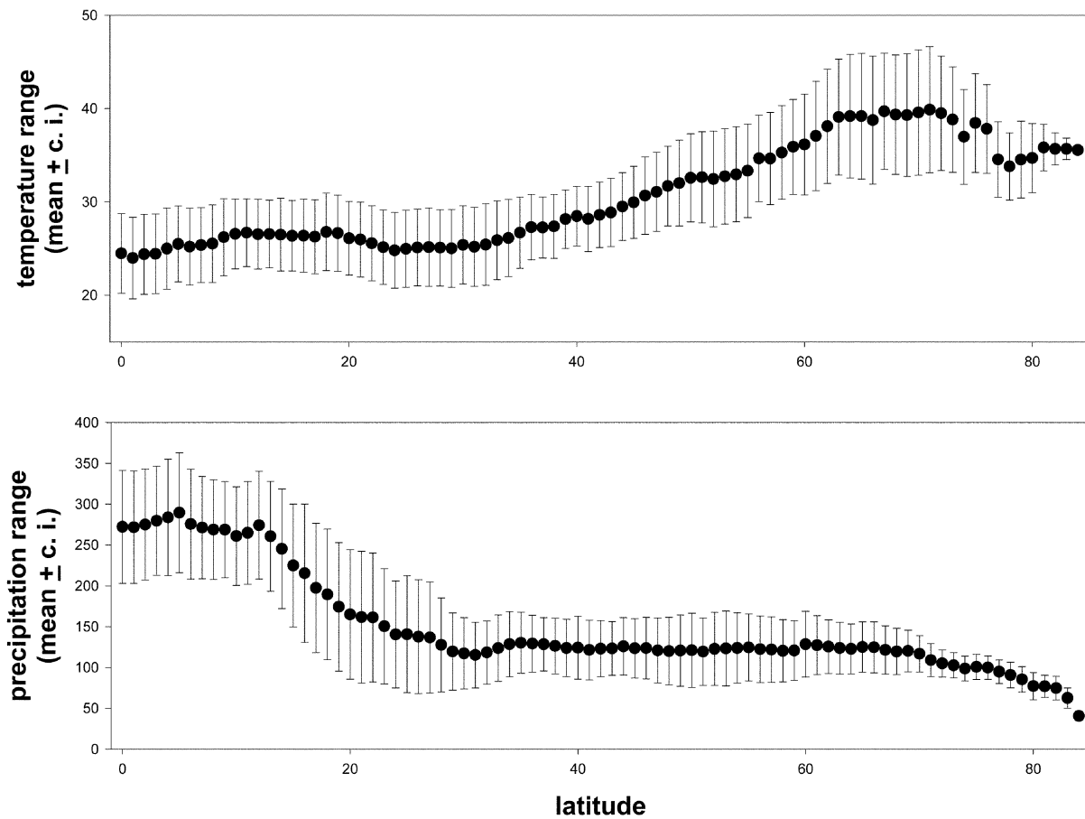
Figure 1: Ranges of temperature and precipitation and their relationship with latitude. Black circles represent the mean range at a particular latitude, and error bars represent confidence intervals. Spearman's rank correlation coefficient: mean temperature range versus latitude: r_s = 0.88 , N = 85 , P < .0001 ; mean precipitation range versus latitude: r_s = -0.86 , N = 85 , P < .0001 . Data from New et al. (1999; available at http://www.geog.ox.ac.uk/~mnew/research/data_download/index.html ).
